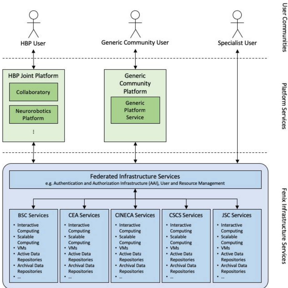
Figure 1: Fenix architecture concept
